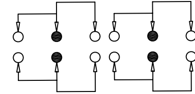
SCHMATIC (NON-SHORTING)
